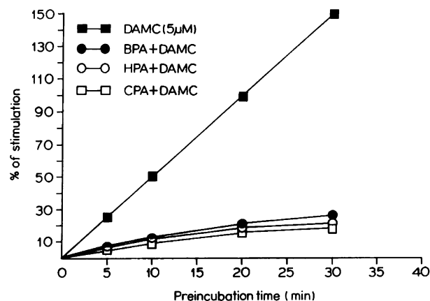
Figure 4. Effect of the inhibitors on the liver microsomal TAase catalyzed activation of NADPH cytochrome C reductase by DAMC. The detailed assay procedure is described under 'Materials and Methods'. The values are the average of three separate observation with error <2%.
