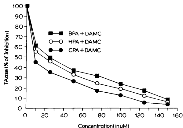
Figure 3. Effect of the concentration of the inhibitors on the activity of TAase. The inhibitors BPA/CPA/HPA at the concentration of 10–150 \mu M were separately included in the reaction mixture of TAase as described under 'Materials and Methods'. The values are the average of three separate observations with error <5%.
