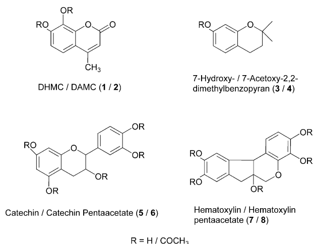
Figure 1. Structures of the substrate and the inhibitors of TAase.
